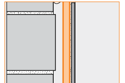
12.1 Schluter®-KERDI-BOARD
