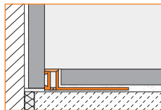
4.9 Schluter®-DILEX-BWA
