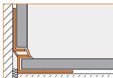
4.13 Schluter®-DILEX-EKE
