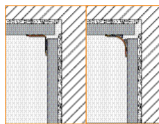
2.7 Schluter®-ECK-KI/-KHK
