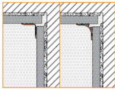
2.7 Schluter®-ECK-KI/-KHK
